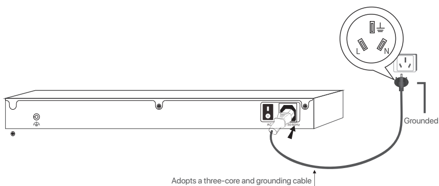
Figure 2-3 Grounding through an PE wire
