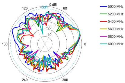
Elevation: 5000 – 6000 MHz
